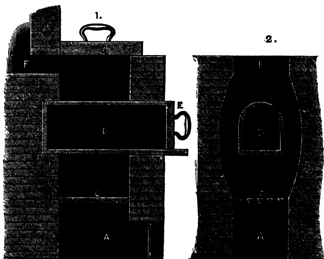
Fig. 138. Nos. 1 and 2, cupelling or enamelling furnace. In both \Delta is the ash-pit, \circ the fire-bars, \square the muffle, \times the opening for introducing the muffle, \nabla the chimney, and \alpha the cover.
